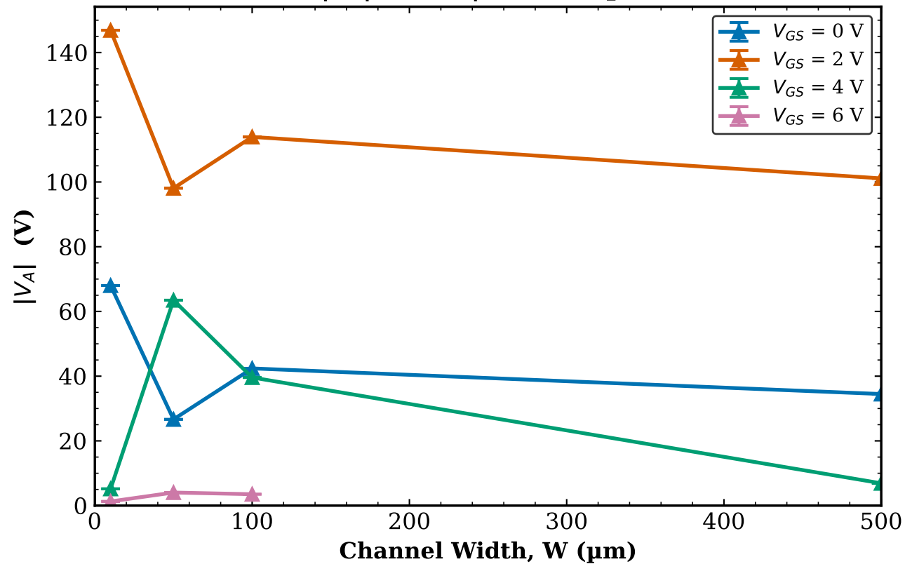
TFT2 Transistor 1 |V_A| vs W | L = 80\text{ }\mu\text{m}
